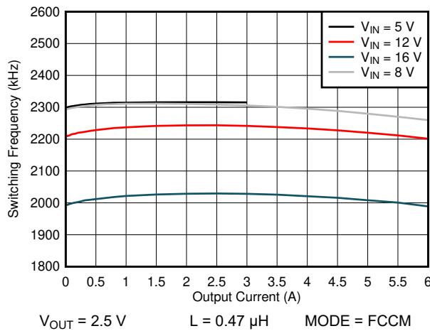
Figure 6-17. 2200 kHz Switching Frequency vs Load Current
