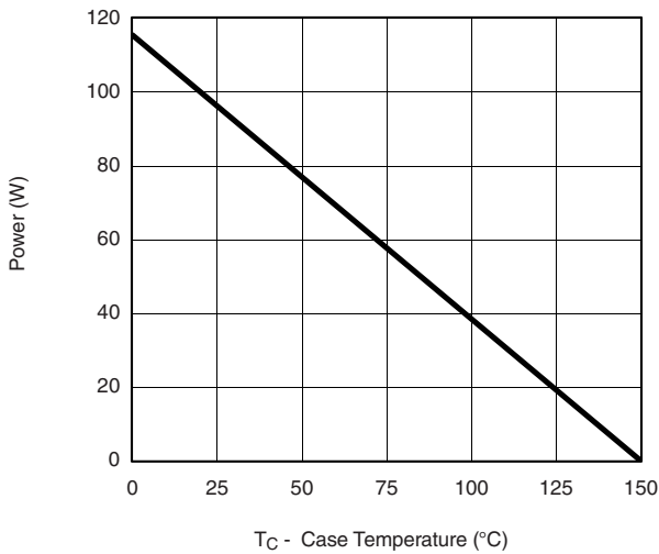
Power, Junction-to-Case
