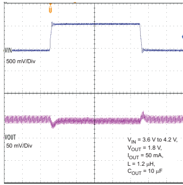
Figure 21. Line Transient PFM Mode
