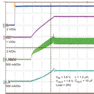
Figure 22. Start-Up into Load – V_{OUT} 1.8 V
