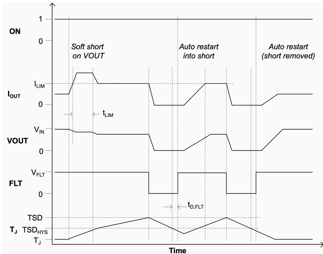
Figure 9-1. Output Current Limit for Short-Circuit Protection ( t_{LIM} )
