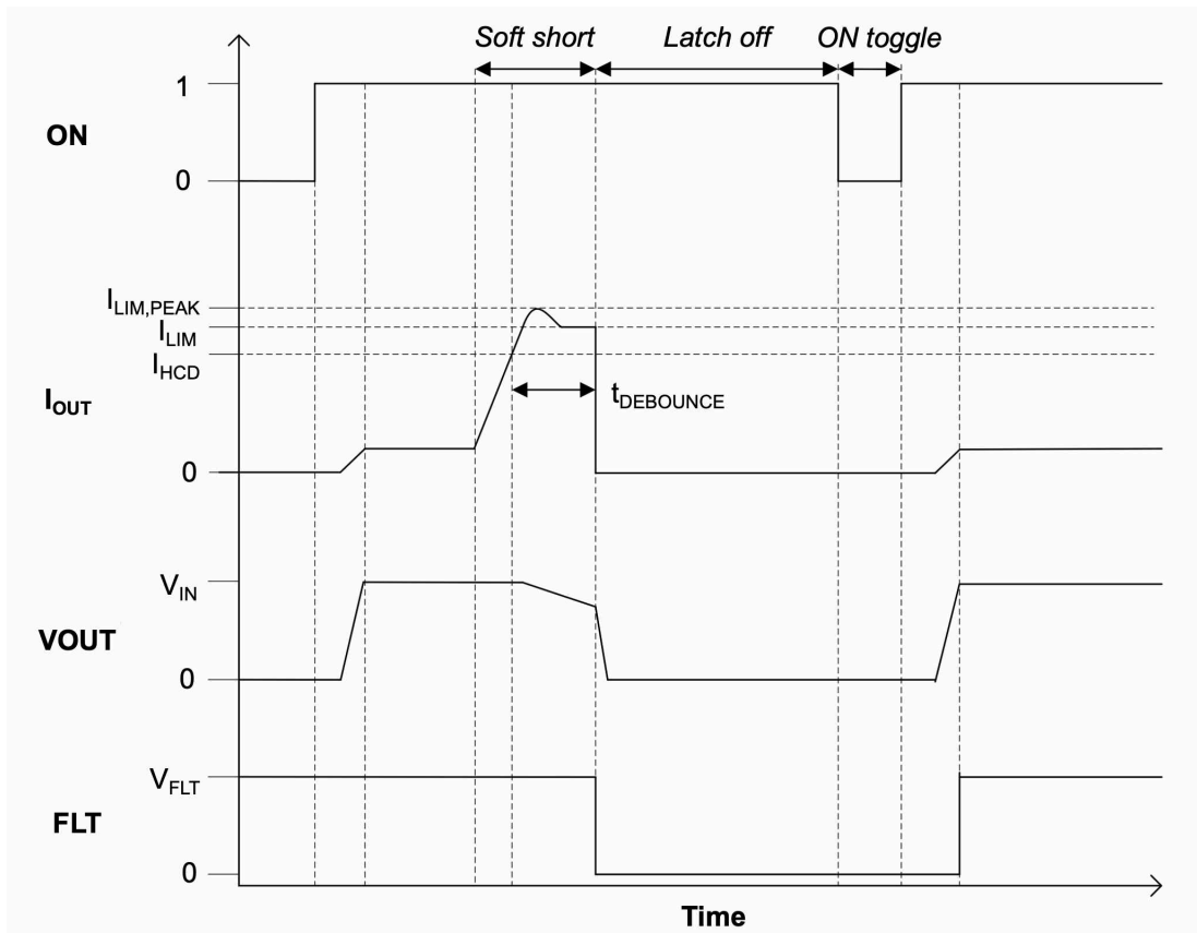
Figure 9-3. Output Current Limit Behavior
