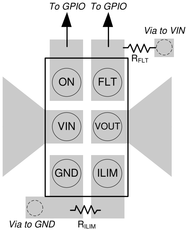
Figure 12-1. TPS22950x Layout Example
