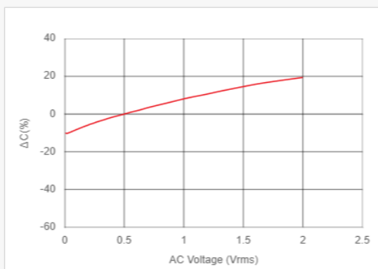
AC Voltage Characteristics LCR meter, 0.12kHz
