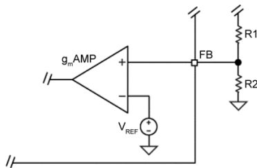
Figure 8. Voltage-Divider Configuration
