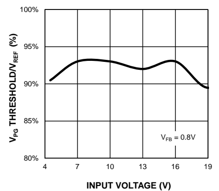
PG Threshold/VREF Ratio vs. Input Voltage
