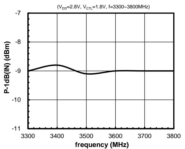
P-1dB(IN) vs. frequency
