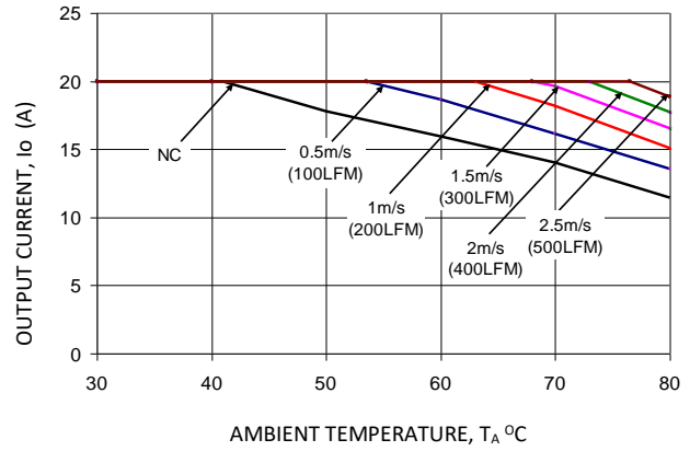
Figure 22. Output Current Derating versus Ambient Temperature and Airflow (ATS020A0X3-SRH).
