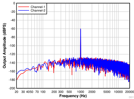
Figure 7-14. FFT With a -60-dBr Input
