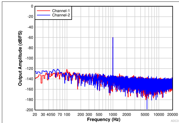
Figure 9-2. FFT With a -60-dBr Input
