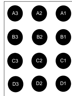
Figure 5. Bottom View
