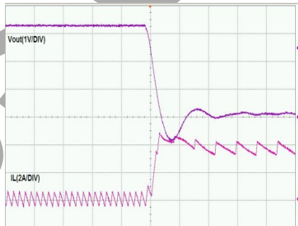
Time -20µs/div
