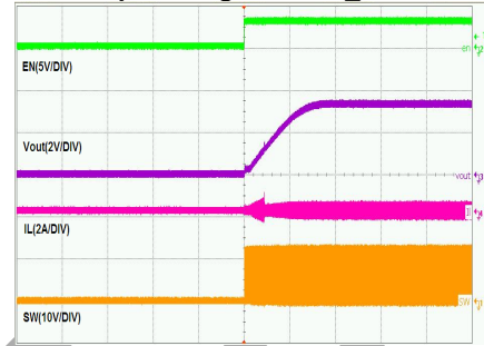
Time -10ms/div
