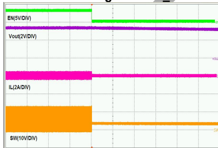
Time -10ms/div
