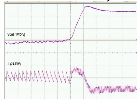
Time -50µs/div
