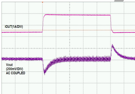
Time -100µs/div
