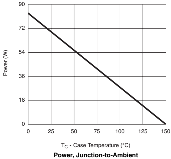
Power, Junction-to-Ambient
