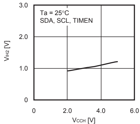
1. 30 High-level input voltage 2 ( V_{IH2} ) vs. Power supply voltage ( V_{CC} )
