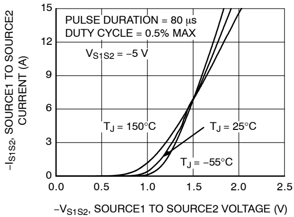
Figure 7. Transfer Characteristics
