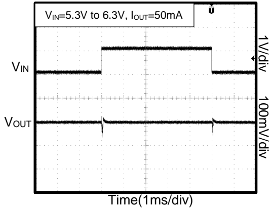
Figure 1. Line-Transient Response
