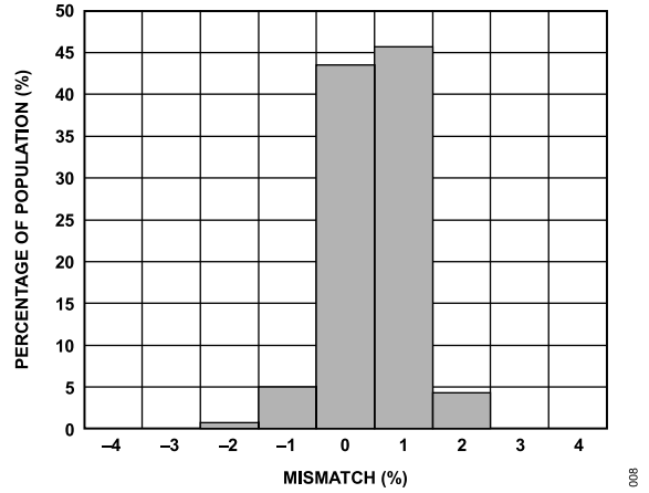
Figure 7. Self-Test Mismatch at 25°C (V_RATIO = 5 V)
