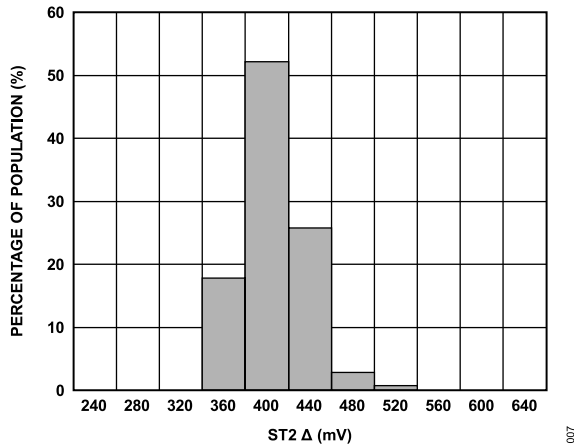
Figure 6. ST2 Output Change at 25°C (V_RATIO = 5 V)
