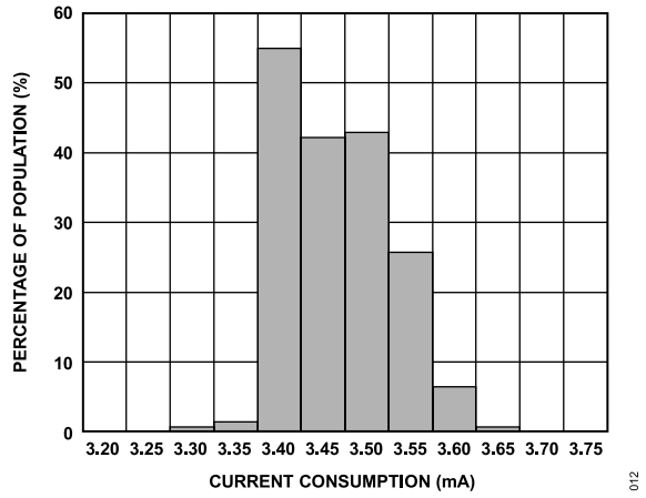
Figure 11. Current Consumption at 25°C ( V_{RATIO} = 5\text{ V} )
