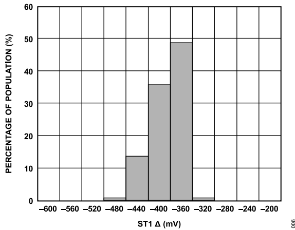
Figure 5. ST1 Output Change at 25°C (V_RATIO = 5 V)
