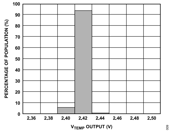
Figure 8. V_TEMP Output at 25°C (V_RATIO = 5 V)
