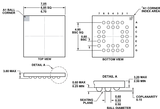
Figure 17. 32-Lead Ceramic Ball Grid Array [CBGA] (BG-32-3) Dimensions shown in millimeters
