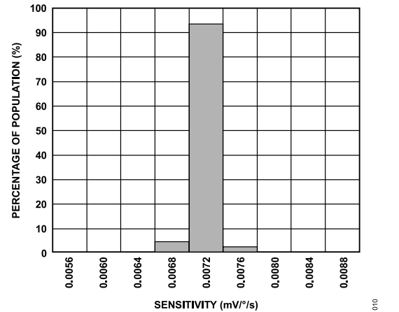
Figure 9. Sensitivity at 25°C
