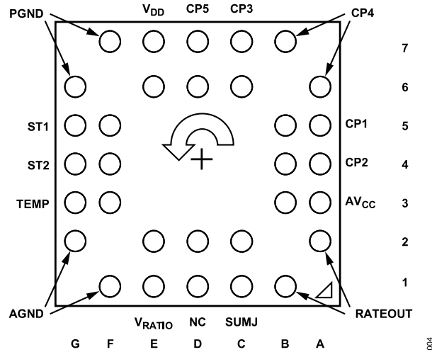
Figure 3. Pin Configuration
