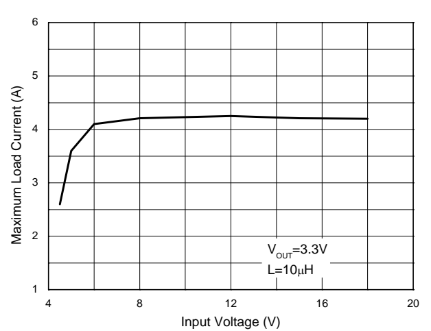
Maximum Load Current vs. Input Voltage
