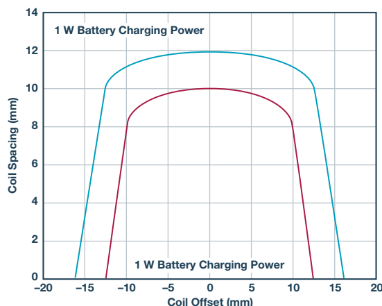
Figure 2. Effect of offset and spacing between the two coils.
