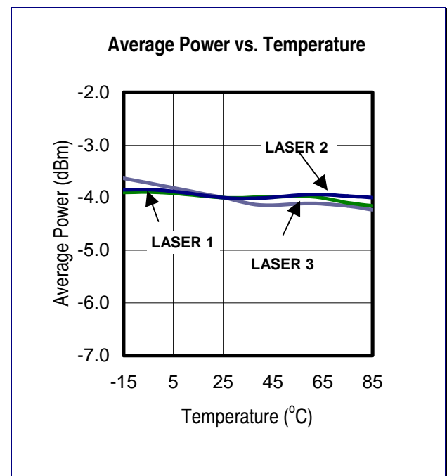
Figure 1: Average Power vs. Temperature
