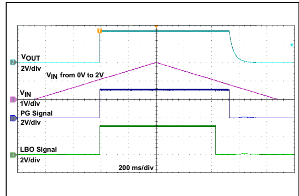
FIGURE 2-42: 3.3V V_{OUT} , UVLO Set for 1.1V.
